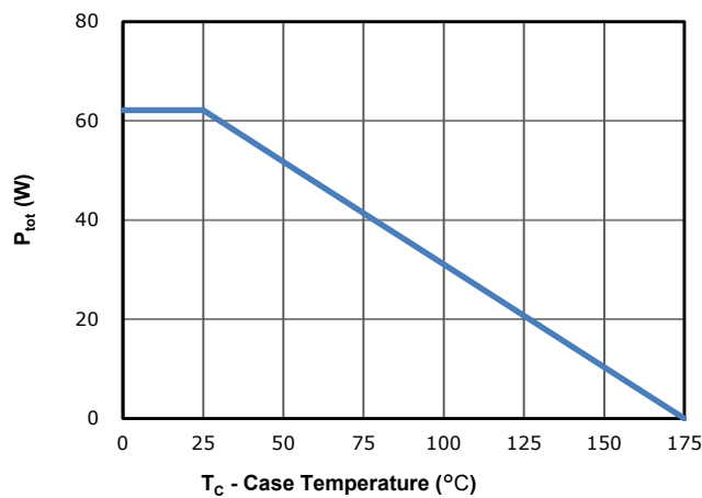
Fig 11: Power Dissipation
